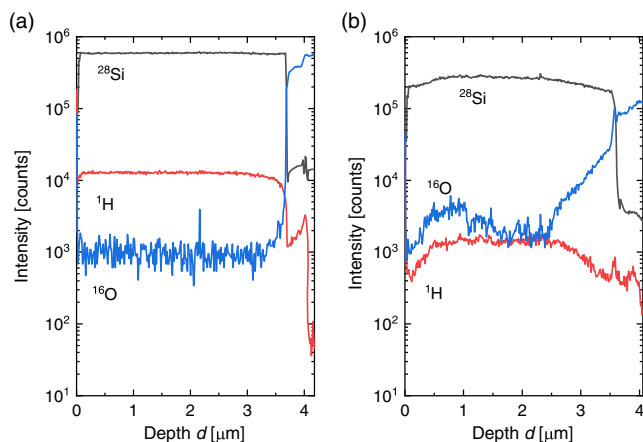
Figure 4. Silicon, hydrogen, and oxygen SIMS depth profiles of thick films of thermally stable a-Si:H, a) as-deposited and b) after annealing (heating schedule see Figure 1) at 550^\circ\text{C} for 5 min.
